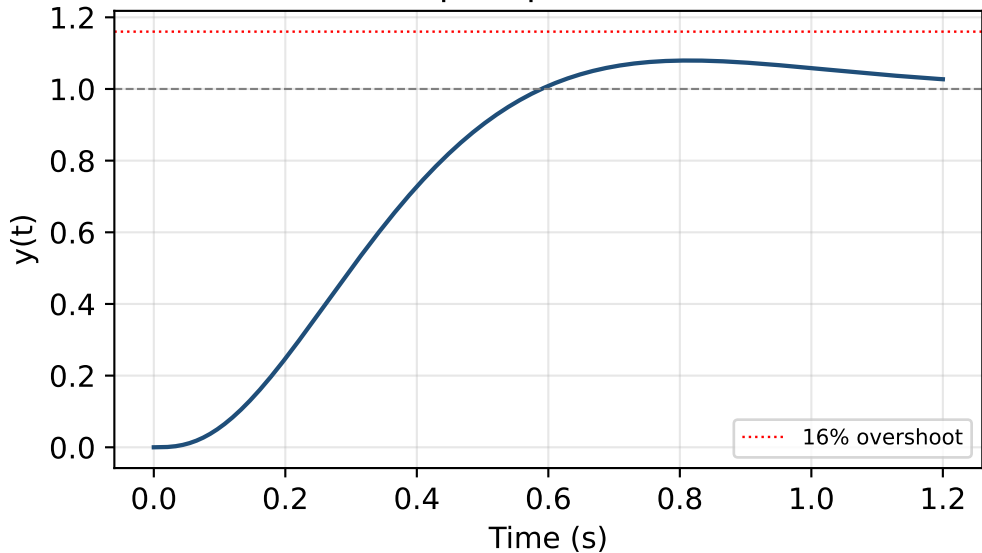
Problem 27: Step response (transient detail)
